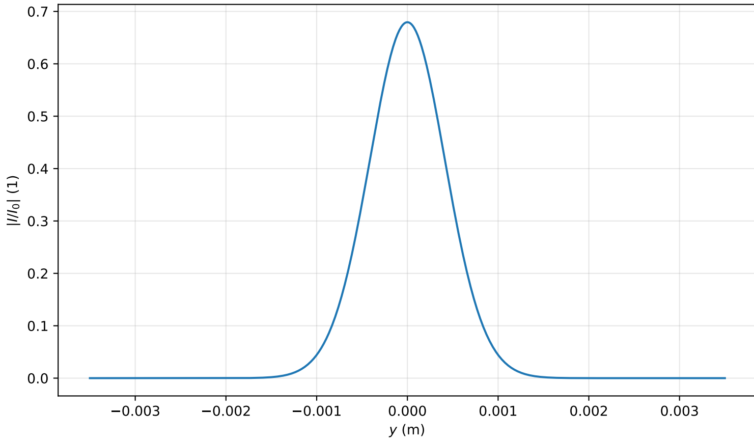
Intensity profile I(x=0, y, z=1.513)/I_0 , P_{in}=0.1P_{cr} , artificial time
